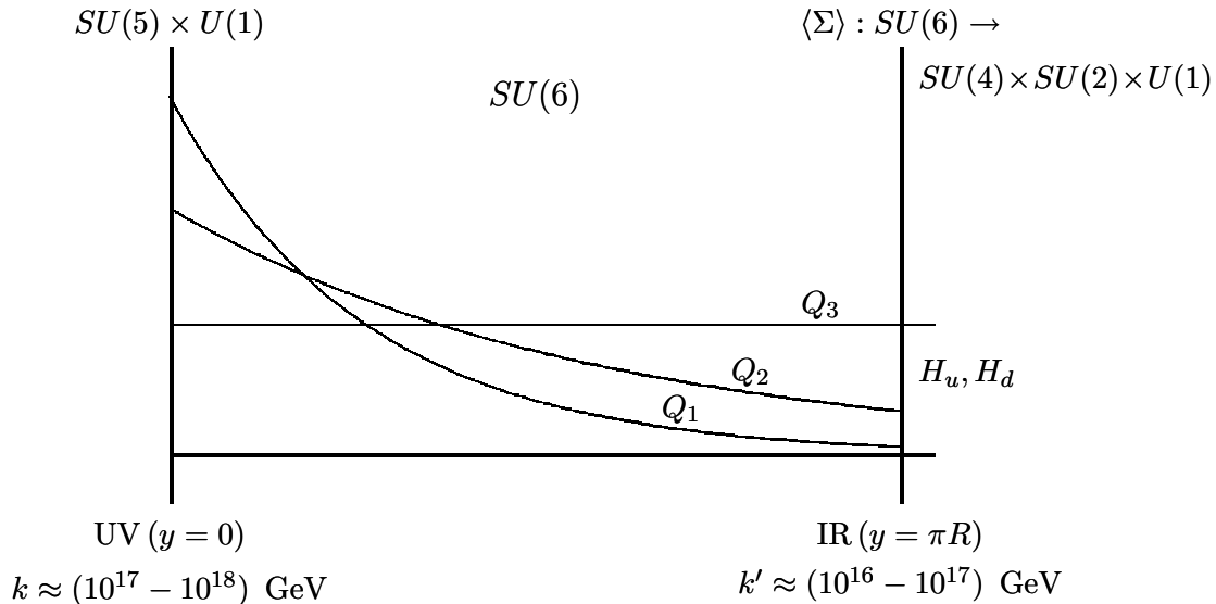
Figure 2: A schematic picture of the model in 5D.
