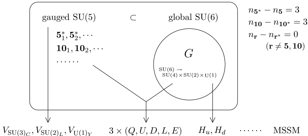
Figure 1: The basic picture of the theory in the 4D description.
